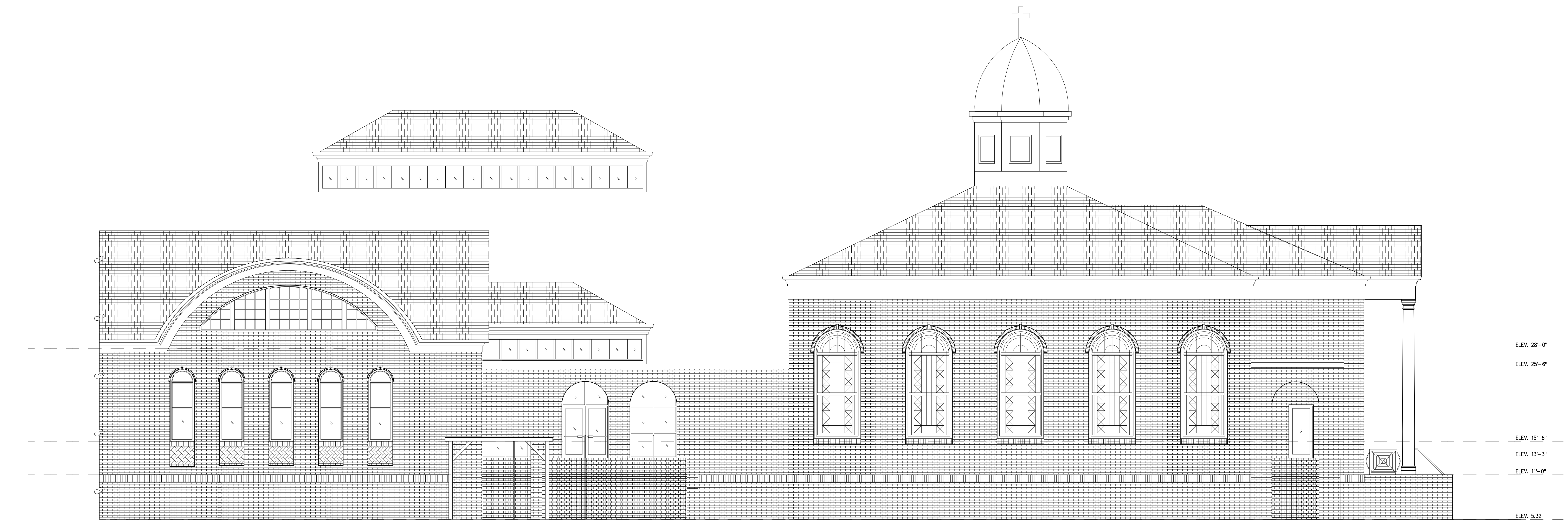
1 A2.4 Partial West Elevation
