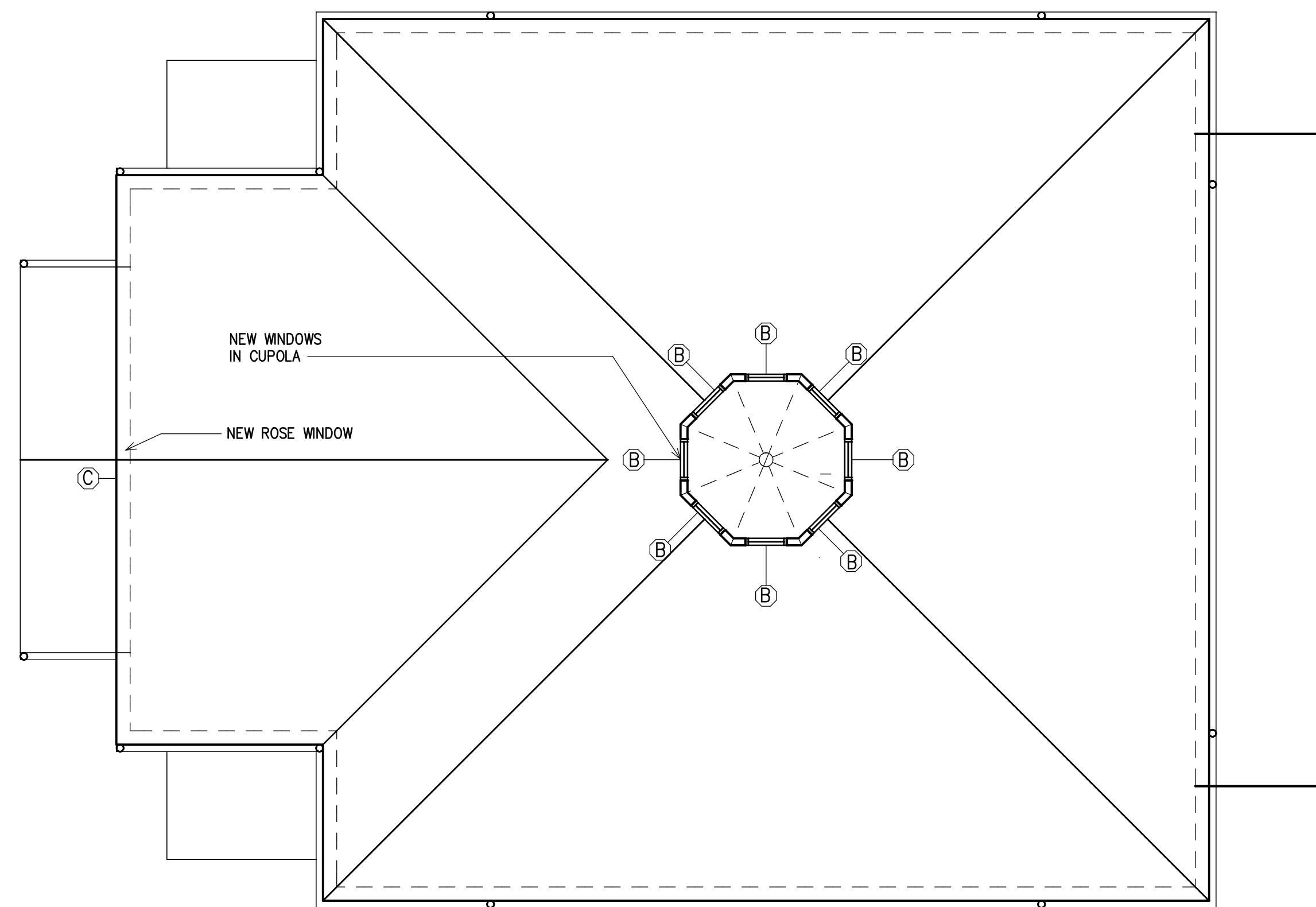
ROOF PLAN 1/8"=1'-0"
