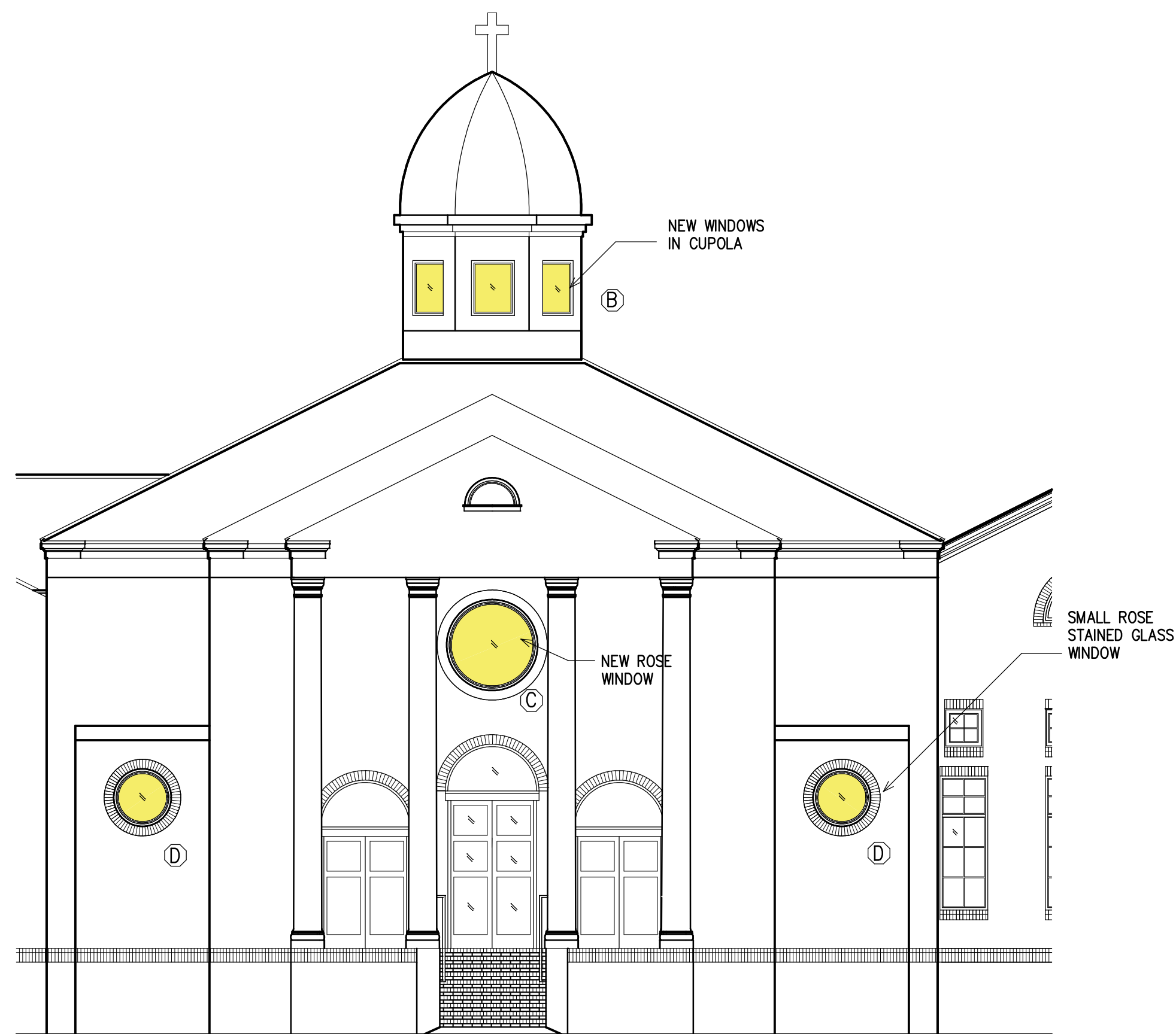
Partial North Elevation 1/8"=1'-0"
