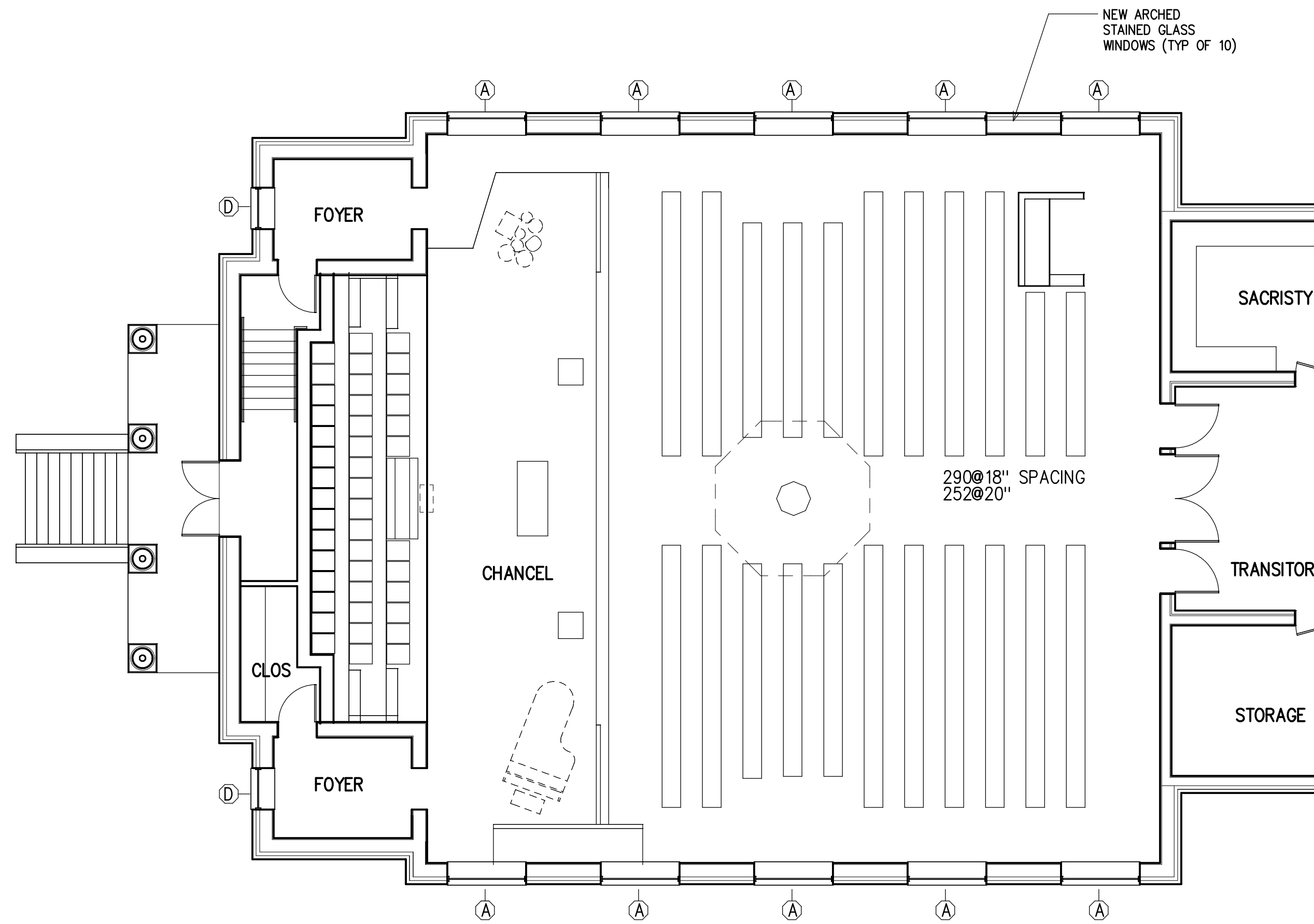
Floor Plan 1/8"=1'-0"
