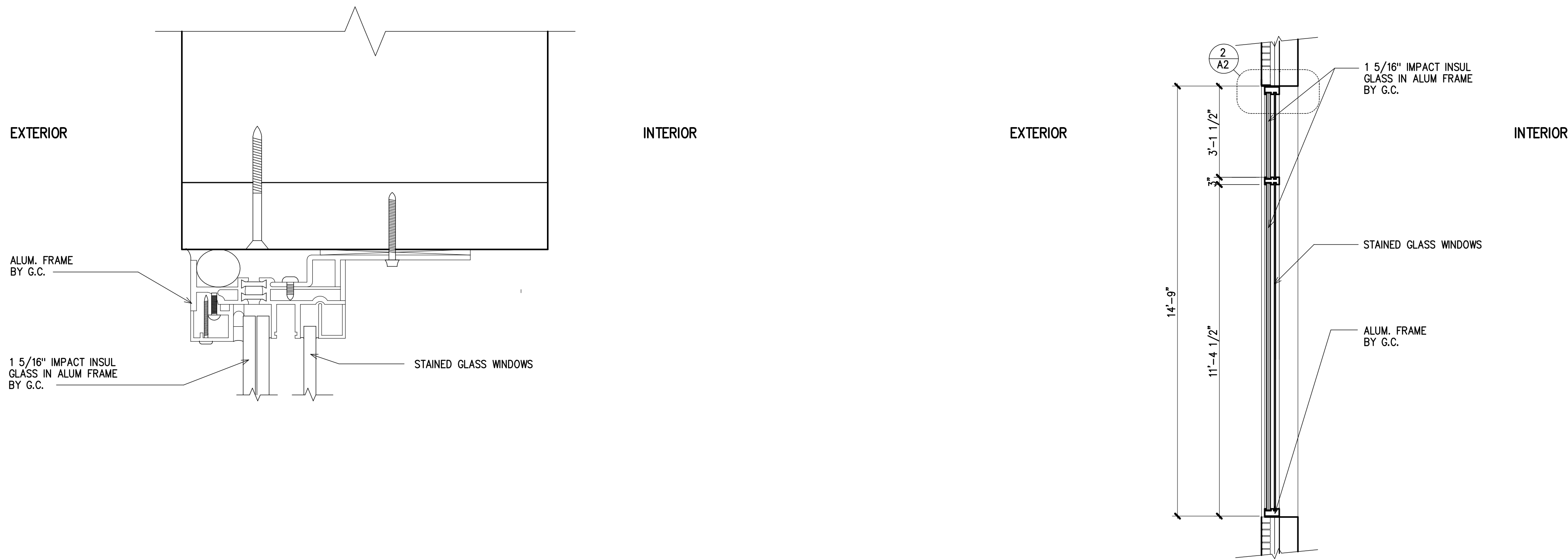
2 A2 Enlarged Detail WINDOW A 3/8"=1'-0"
