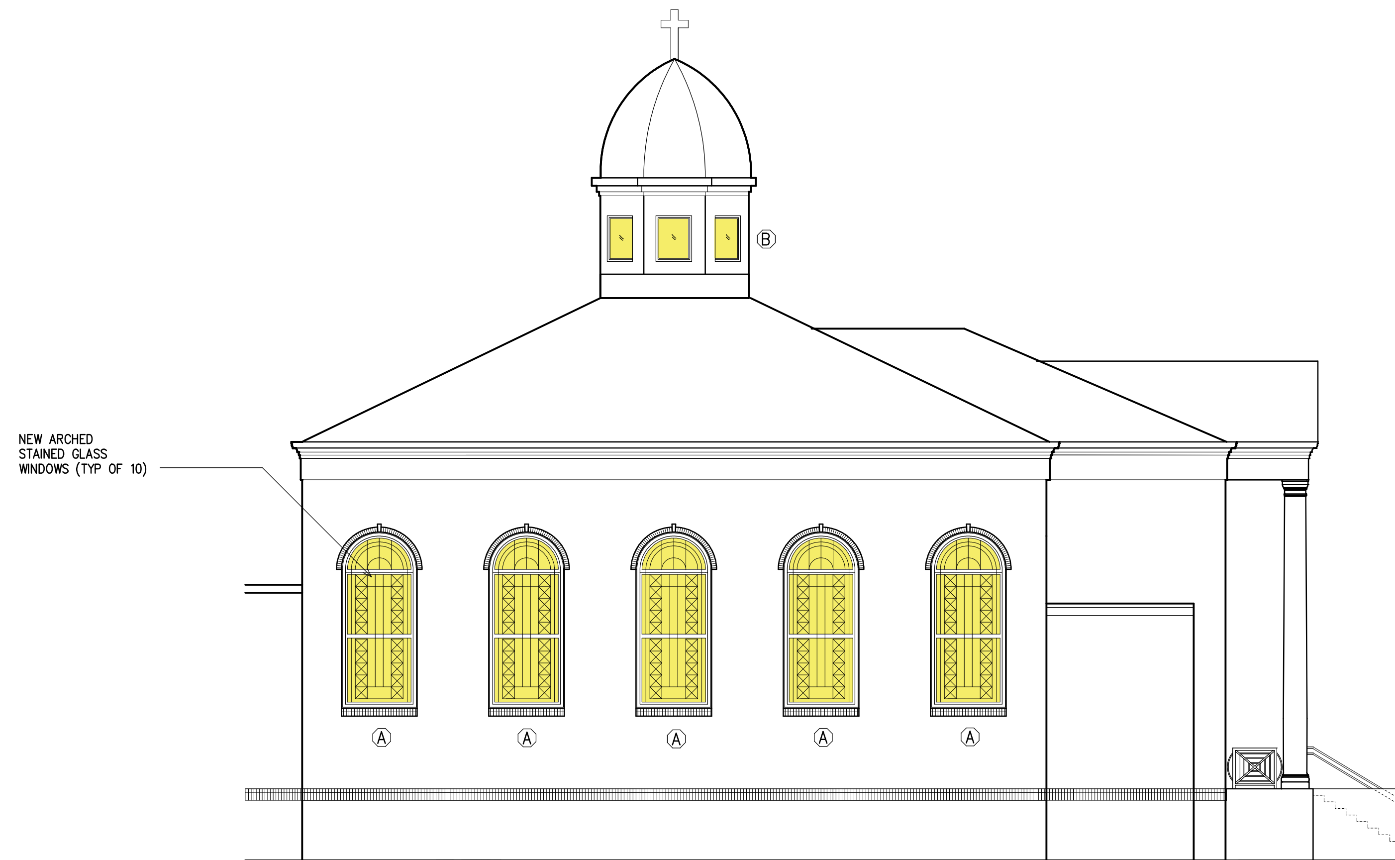
Partial East Elevation 1/8"=1'-0"
